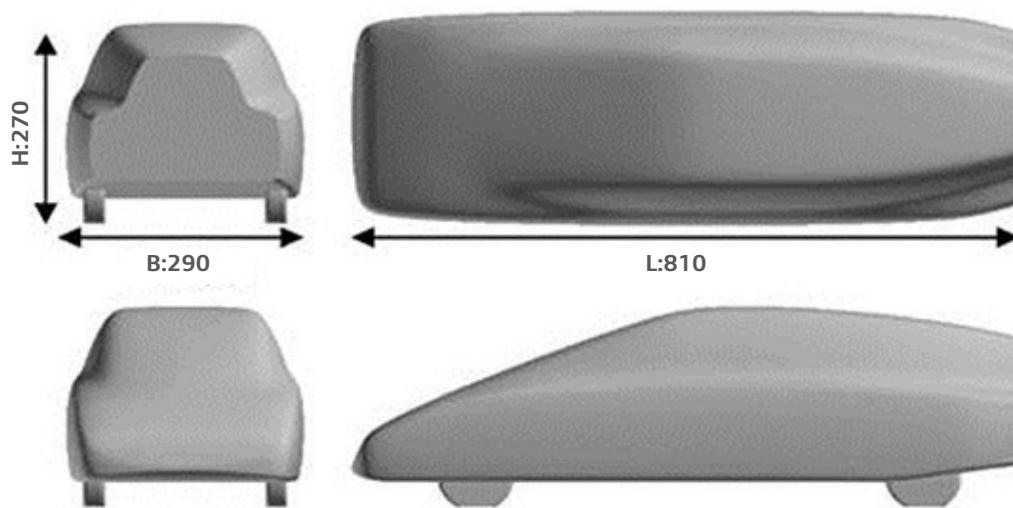
Figure 6: ASMO model geometry (dimensions are in mm).
