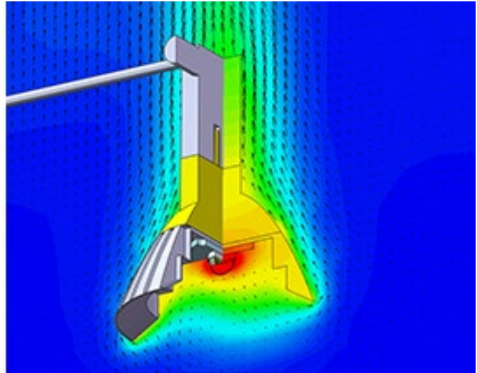
Figure 7: Temperatures on a 2D slice through the center of the lamp with vectors showing flow caused by natural convection over the outside of the lamp.
