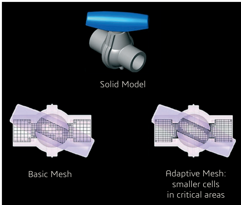
Figure 2: Using a rectangular adaptive mesh, Concurrent CFD tool SOLIDWORKS Flow Simulation can automatically adjust cell size to deliver better resolution anywhere it is needed.
